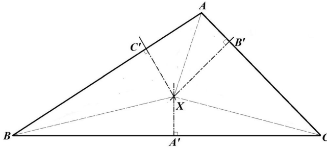
Figure 2. Carnot's Theorem.
