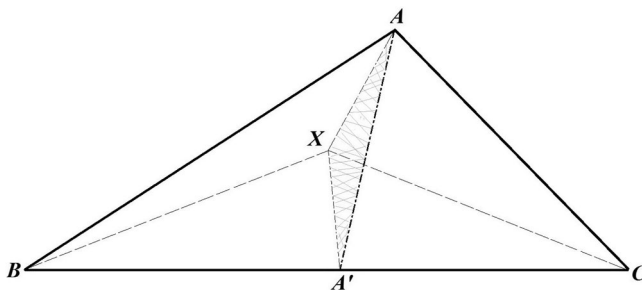
Figure 3. X lies on AA' \iff S_{\triangle AXA'} = 0 .
