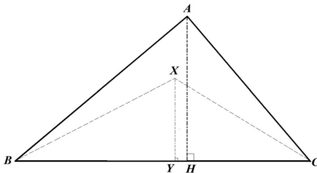
Figure 1. X lies on AH \iff Y = H .
